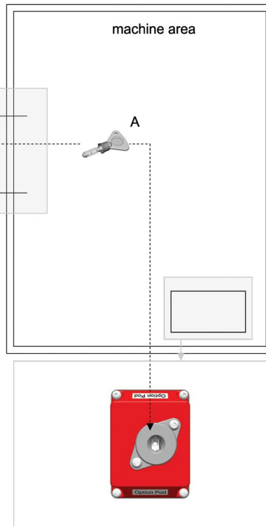
PODK : key option pod for activating teach mode located inside the safeguarded area.
